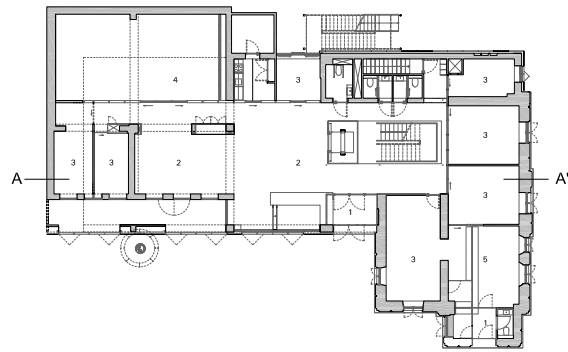
floor plan ground floor
